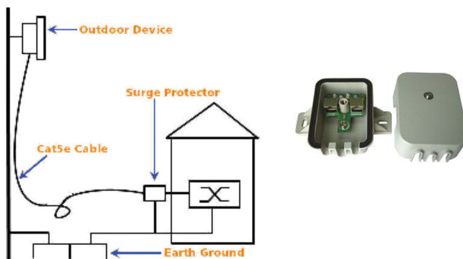
Figure 4-6 Surge Protector
