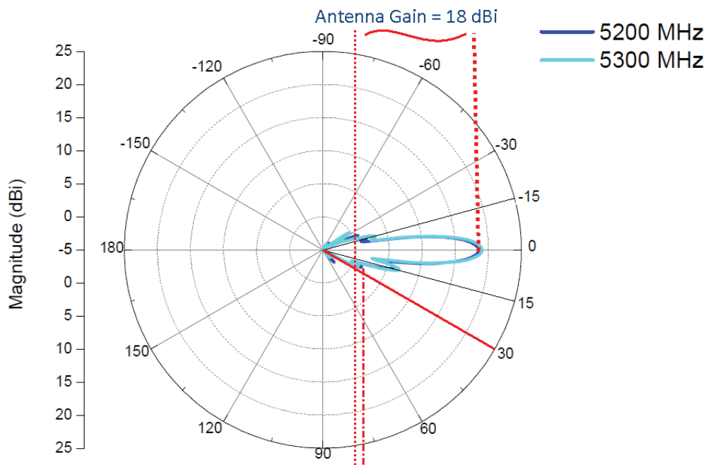
Figure 8-4 Antenna gain at (30 - \theta) = 30^\circ
