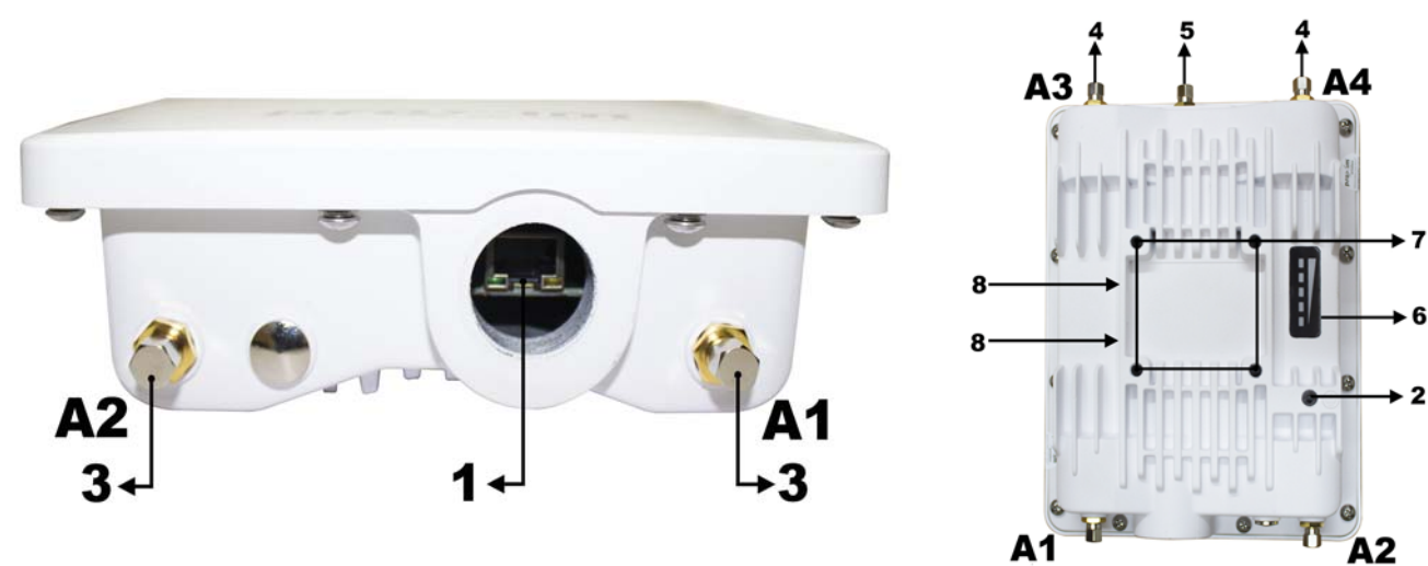
Figure 3-1 MP-10x5-CPE, MP-10x5-BS3 & QB-10x5-EPR
