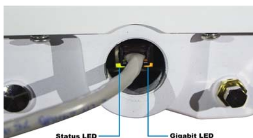
Figure 4-8 Port LED Indicators
