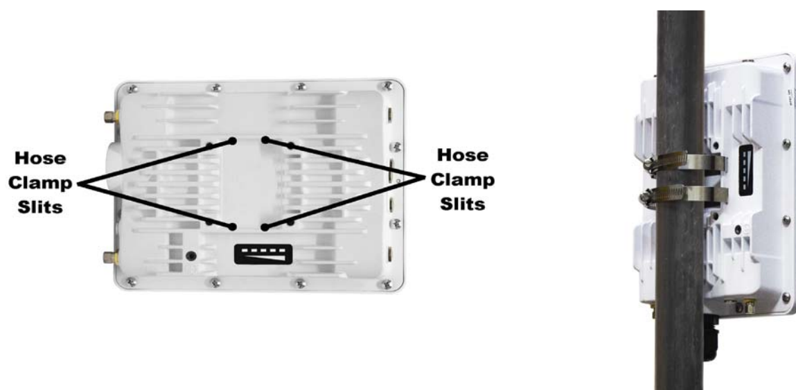
Figure 4-4 Pole Mounting (MP-1035)
